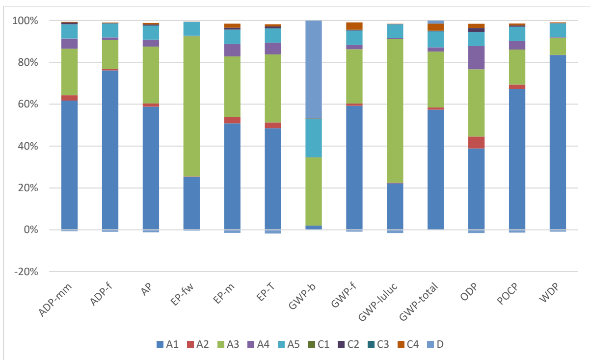
Figure 2: LIP Folie G35 - Impact of the individual modules on the environmental core indicators
